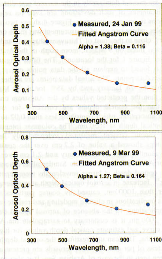
Figure 4. Examples of the measured aerosol optical depth values, curve fitted using eq. (1). The optical depth at 1050 nm is seen falling outside the fitted curve on several occasions during the cruise.
