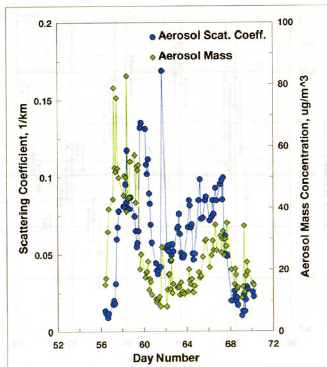
Figure 9. Comparison of aerosol mass concentration (accumulation mode) and scattering coefficient obtained over the Arabian Sea and the coastal region. The ratio of aerosol scattering coefficient to aerosol mass is found to be 2.27 \text{ m}^2/\text{g} .
