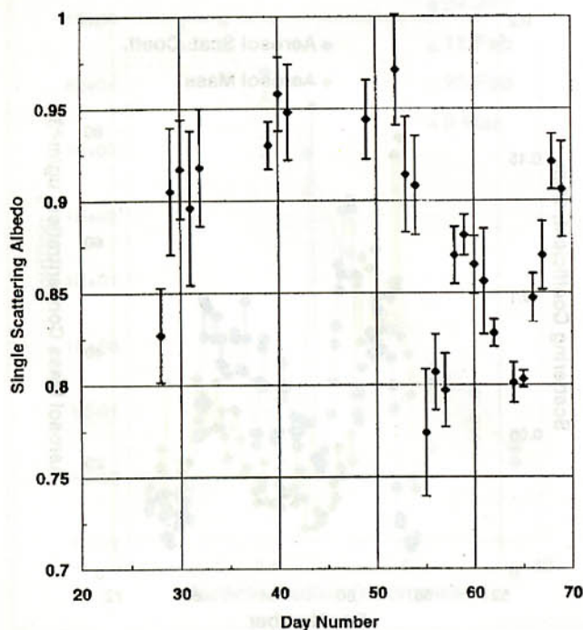
Figure 10. Single scattering albedo \omega , obtained from the daily averaged aerosol scattering and absorption data. Vertical bar shows one standard deviation of the mean. The uncertainty in the computed \omega values is less than \pm 2.5\% for \omega > 0.9 and between \pm 2.5\% and \pm 5\% for 0.8 < \omega < 0.9 .
