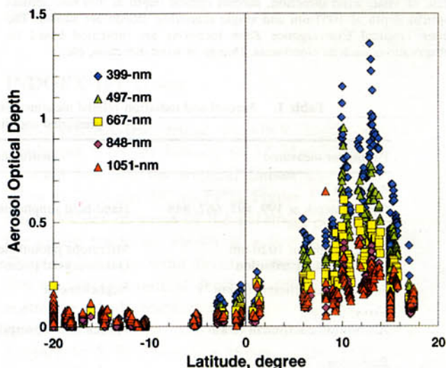
Figure 2. Aerosol optical depths, measured along the cruise track, are plotted as a function of latitude to show the large north-south asymmetry seen in the values. The latitude gradient persists from north down to about 5^\circ\text{S} , where the ITCZ was located.
