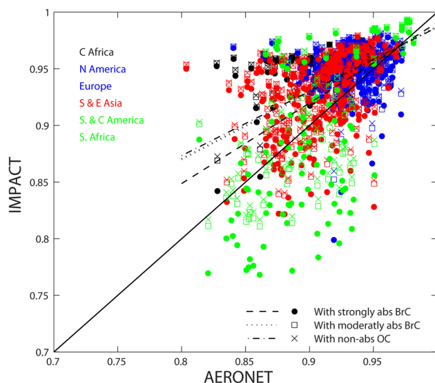
Fig. 4. Comparison of monthly mean SSA at 550 nm from AERONET (1992–2011) and three model simulations (NON, MOD, and STR). The solid line indicates the 1 : 1 ratio. Data points in central Africa (C. Africa), Europe and North America, South Asia and East Asia (S & E Asia) and regions dominated by biomass burning (South and Central America (S & C America) and southern Africa (S. Africa)) are colored in black, blue, red, and green, respectively. The linear fitting functions are y = 0.71x + 0.3 for the STR BrC (dashed line; solid circles), y = 0.58x + 0.4 for the MOD BrC (dotted line; open squares), and y = 0.57x + 0.42 for the non-absorbing OC (dash-dotted line; cross symbols).
