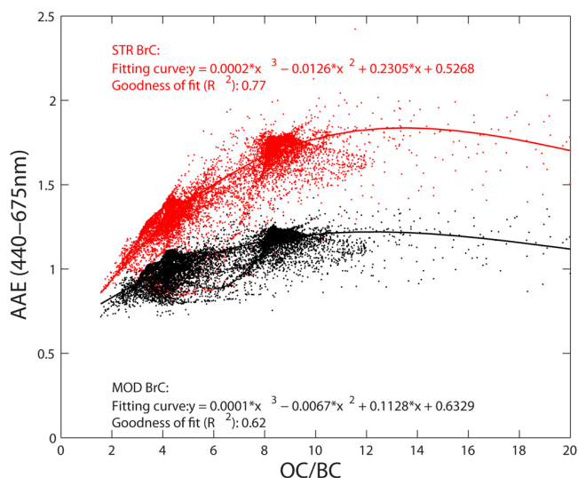
Fig. 7. The simulated wavelength dependence of AAE (440–675 nm) as a function of the ratio of OC : BC column burden, for the STR BrC and MOD BrC. The fitted curves are valid for ratios of OC : BC between 1.5 and 20.
