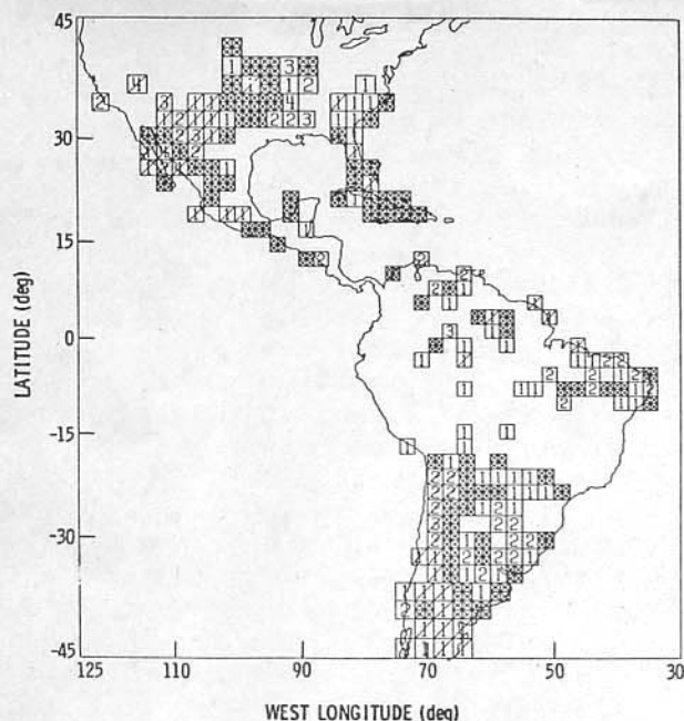
FIG. 2. Differences between nearly simultaneous Nimbus-7 and GOES-derived regional, broadband albedos in % for land area during November 1978 for cloud fractions <10%. (Shaded areas indicate differences within \pm 0.5\% . Numbers with slashes indicate that Nimbus-7 values are less than GOES. Blank areas indicate nearly cloud-free data were not available.)
