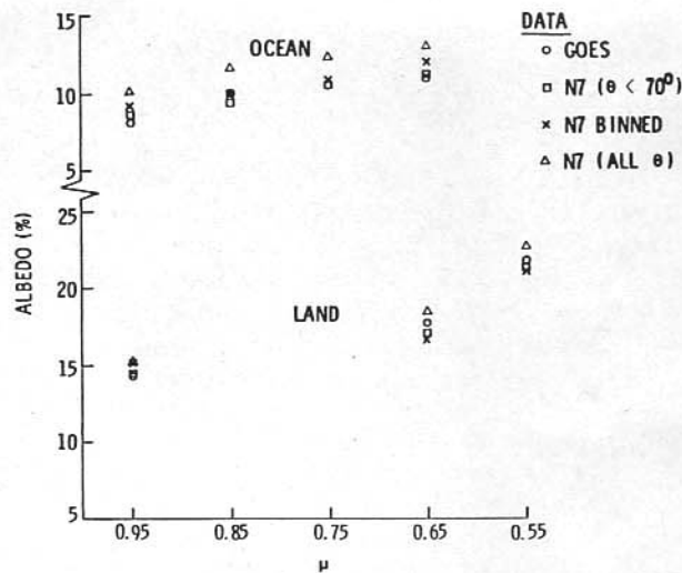
FIG. 1. Comparison of mean ocean and land clear-sky albedos derived from nearly simultaneous Nimbus 7 and GOES data for cloud fractions < 10\% during November 1978.
