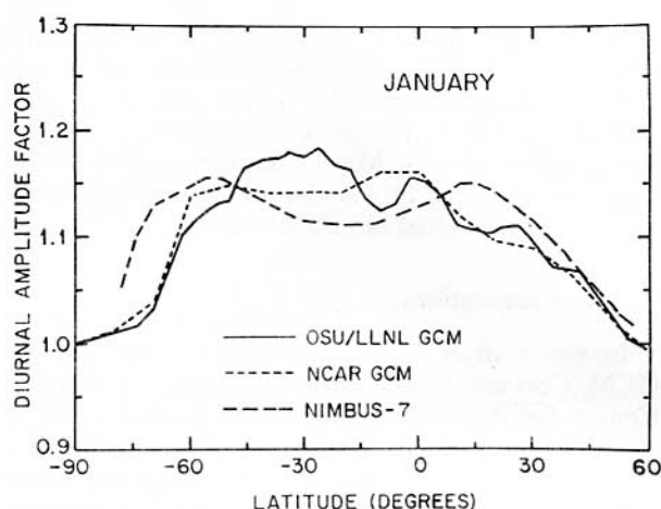
FIG. 8. Diurnal amplitude factors for January. These refer to all longitudes.
