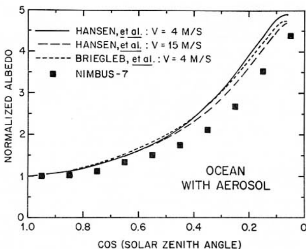
FIG. 3. Directional planetary albedos as evaluated from the solar radiation model using both Hansen et al. (1983) and Briegleb et al. (1986) albedo models for the ocean surface. Also shown are Nimbus-7 (Taylor and Stowe, 1986) measurements.
