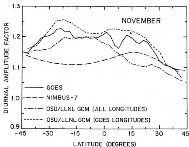
FIG. 6. Diurnal amplitude factors for November.
