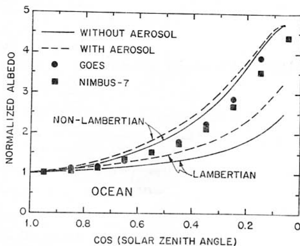
FIG. 2. Directional planetary albedos as evaluated from the solar radiation model both with and without maritime aerosols, and with and without the assumption of a Lambertian surface. Also shown are satellite results determined from both GOES (Minnis and Harrison, 1984) and Nimbus-7 (Taylor and Stowe, 1986) measurements.
