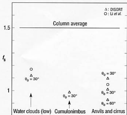
Fig. 3. Comparison of the value for f_s inferred in this study with computed values (31) for different cloud types and for two different radiation models: DISORT and Li et al. (12). Low clouds in the DISORT code have tops at 3 km and bases at 1 km with an effective radius of 10 \mu\text{m} . The cirrus clouds are 1 km thick with tops at 10 km, and the anvils are 3 km thick with tops at 12 km. The cumulonimbus clouds are 6 km thick with tops at 12 km. The effective particle radius in DISORT is 50 \mu\text{m} for all clouds except low clouds. We use a modified gamma distribution function for equivalent spheres. The spectrum ranges from 0.2 to 4.0 \mu\text{m} ; \theta_0 is the solar zenith angle. From the Li et al. model (12), we used ERBE albedos and ship sondes as input.
